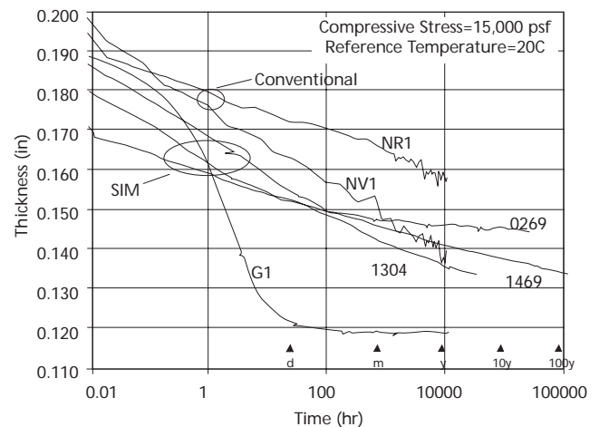
Figure 2. SIM Testing of geonet thickness.
