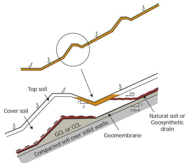
Figure 1. Final cover side slope drain.
