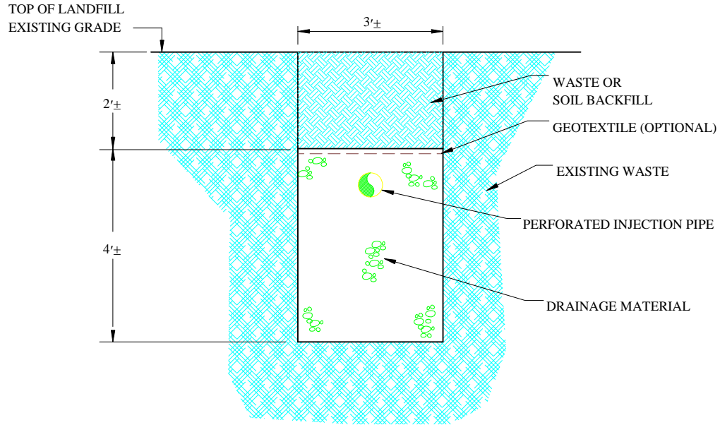
Figure 1. Typical Leachate Injection Trench
