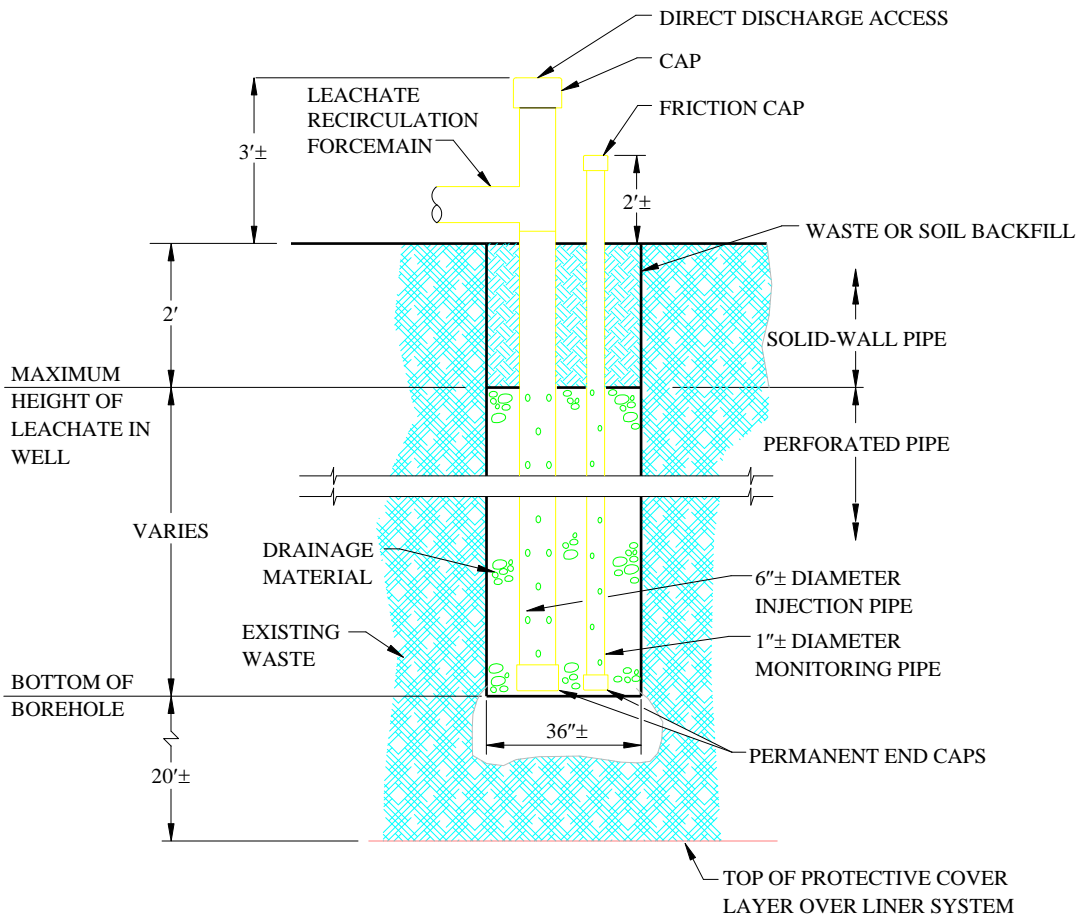
Figure 2. Typical Leachate Injection Well
